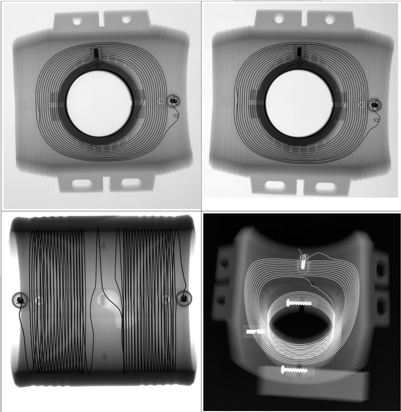
ABS pipes – around 12 cm diameter GemX-160 + DeReO WA-P
